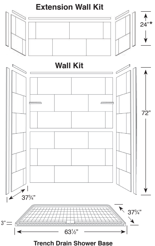
Shown with FG6338 Shower Base, X6382 Extension Wall Kit, GB3729PS Grab Bar Set, H2513 Shower Seat, GBHS18PS Hand Shower with 18" ADA grab bar.
